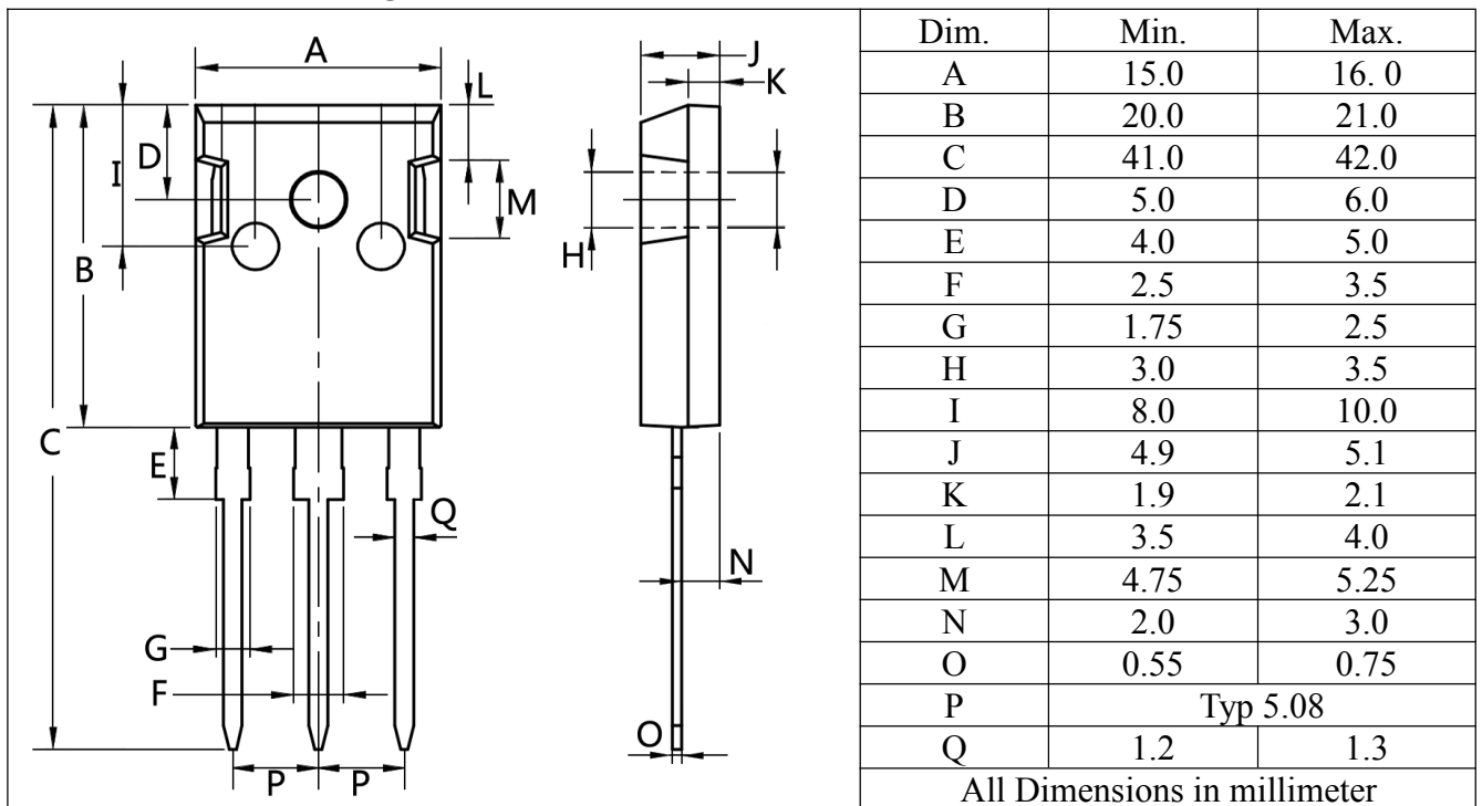
TO-247 封装尺寸 Package size
